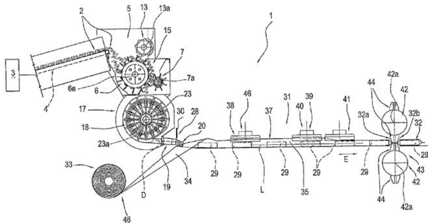
US Patent No: 8,939,157 Method of packaging tobacco
