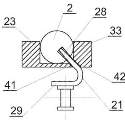
US Patent No: 8,967,370 Unit for conveying filter segments
