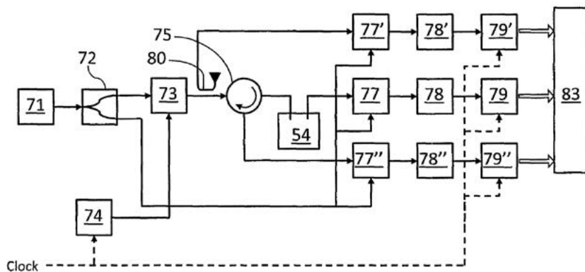
US Patent No: 8,912,805 Device and method for processing and measuring properties of a moving rod of material
